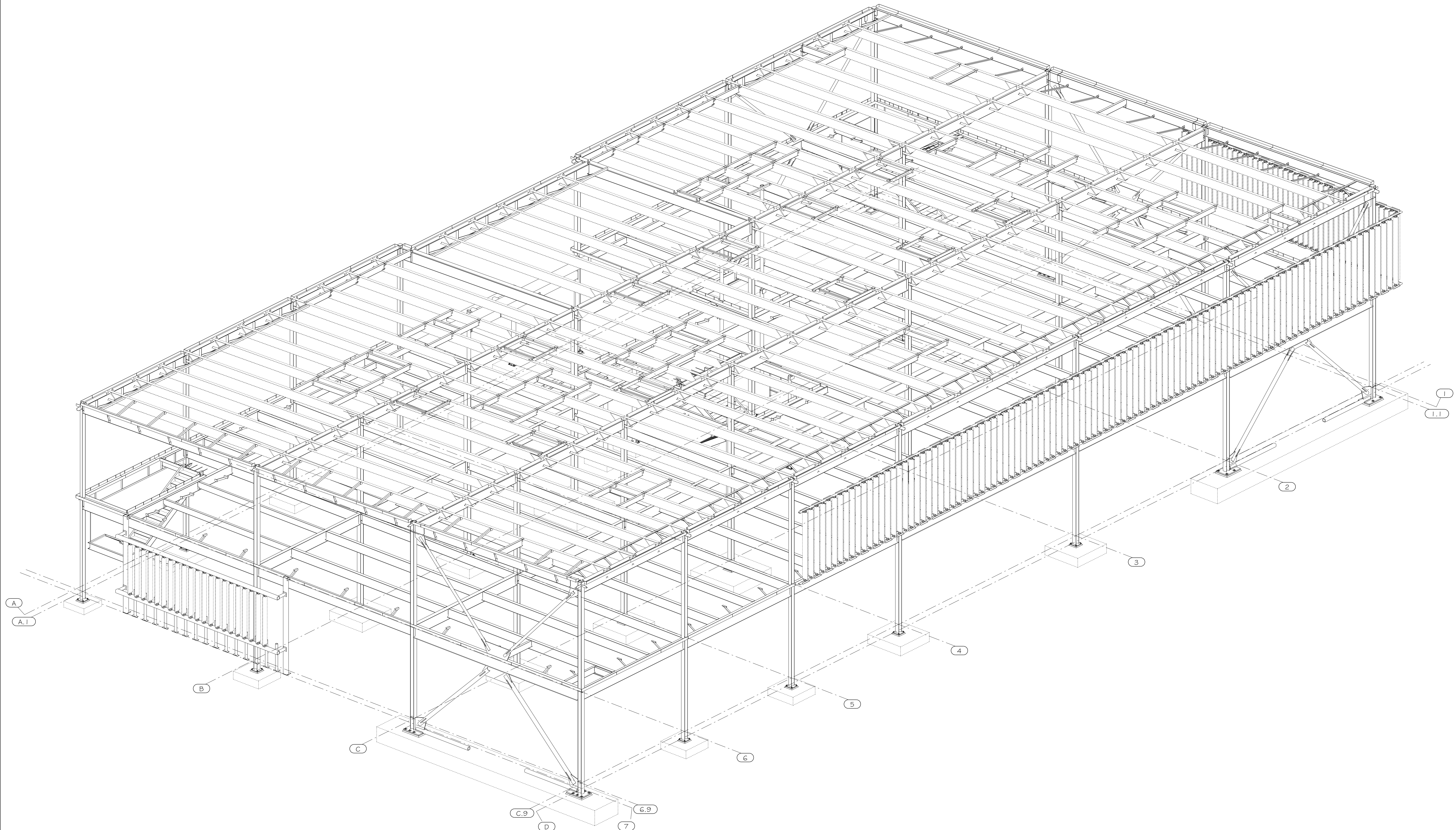
ISO VIEW REFERENCE ONLY
